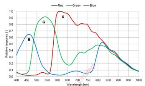
MV-CH120-11UC 量子效率
