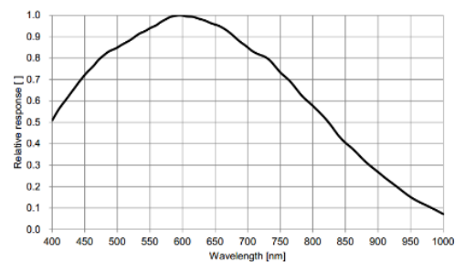
MV-CH120-11UM 量子效率
